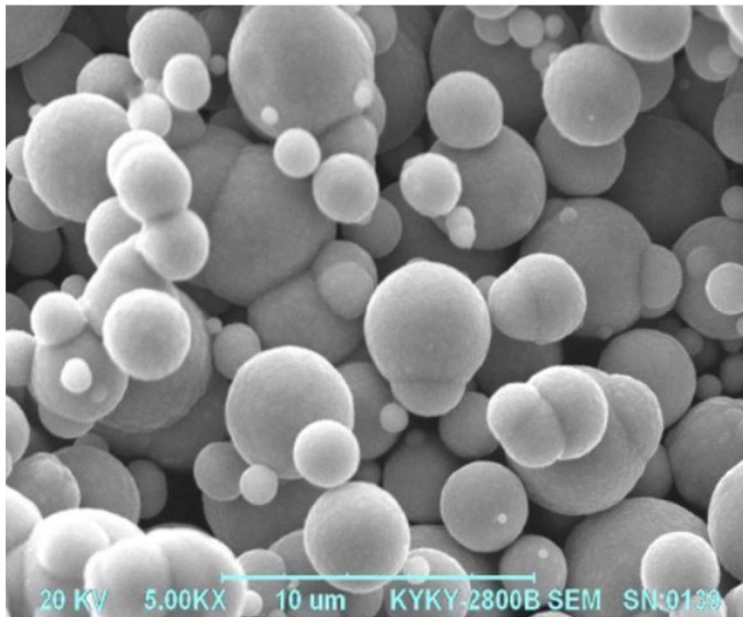
SEM of Carbonyl Iron Powder
